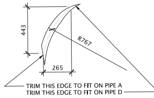
Steel Pipe C Bending Radii
