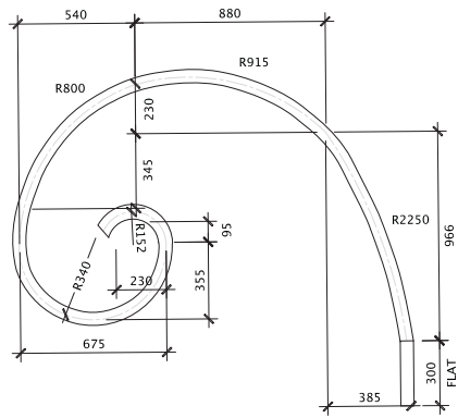
Steel Pipe A Bending Radii
