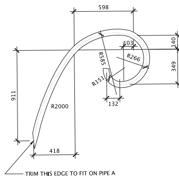
Steel Pipe B Bending Radii
